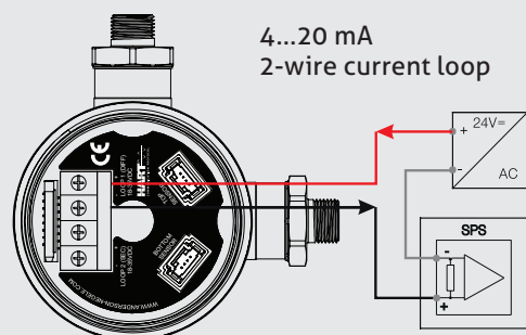
Electrical connection with cable gland
