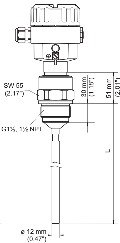
Rod ø 12 mm Process connection: thread, without temperature adapter (80°C/150°C)
