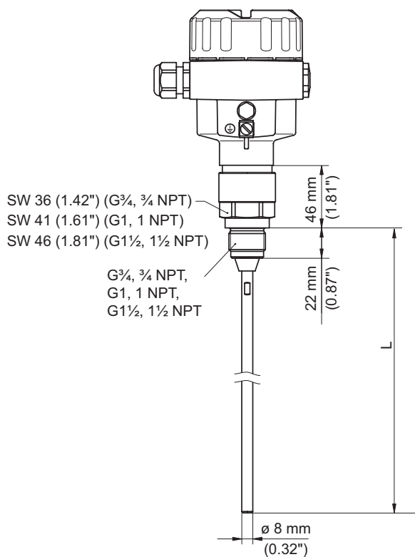
Rod ø 8 mm Process connection: thread, without temperature adapter (80°C/150°C)
