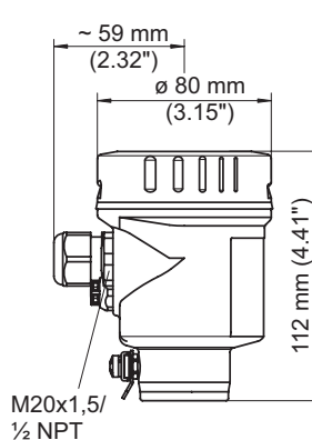
Stainless steel single chamber
